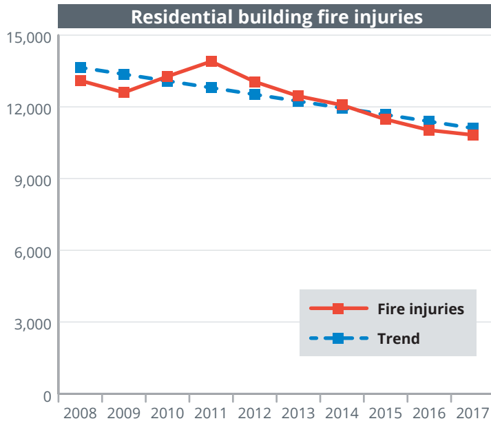
Figure 5. Trends in residential building fires and fire losses (2008-2017) — continued
